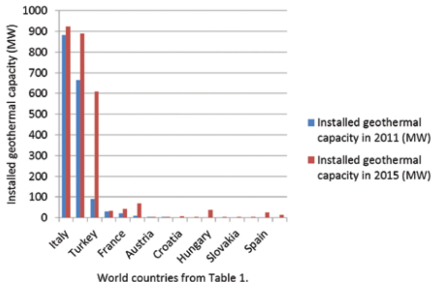
Diagram 2. Histogram showing how the country increased installed geothermal capacity (MW) from 2011 to 2015
